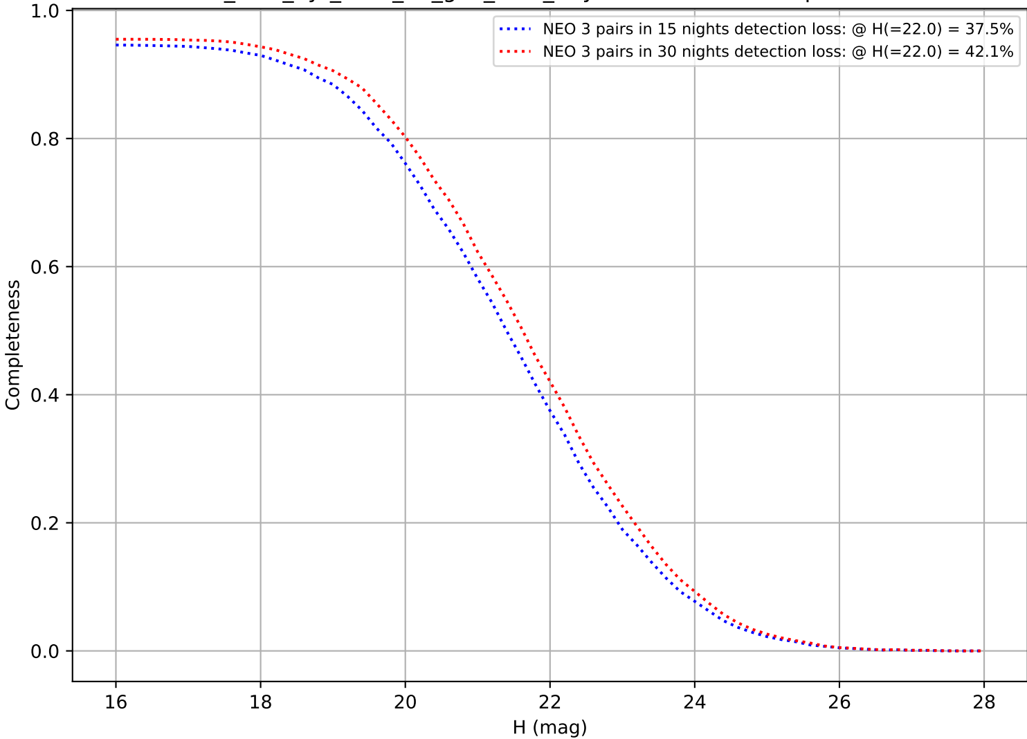
too_elab_2yr_r128_d3_griz_v3.4_10yrs: DifferentialCompleteness
