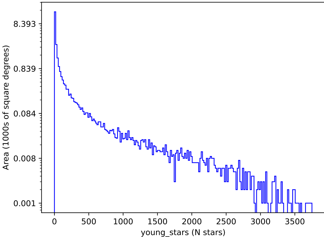
too_elab_2yr_r128_d3_griz_v3.4_10yrs : young_stars
