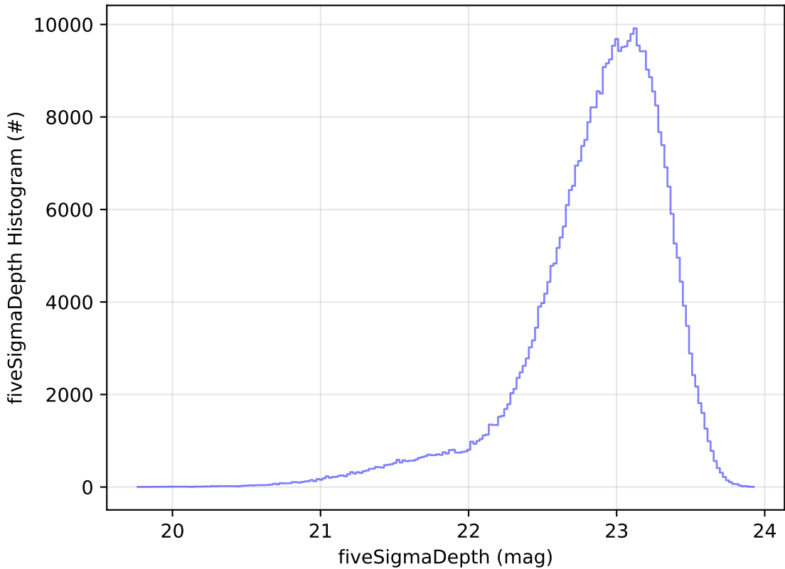
too_elab_2yr_r128_d3_griz_v3.4_10yrs z: fiveSigmaDepth Histogram
