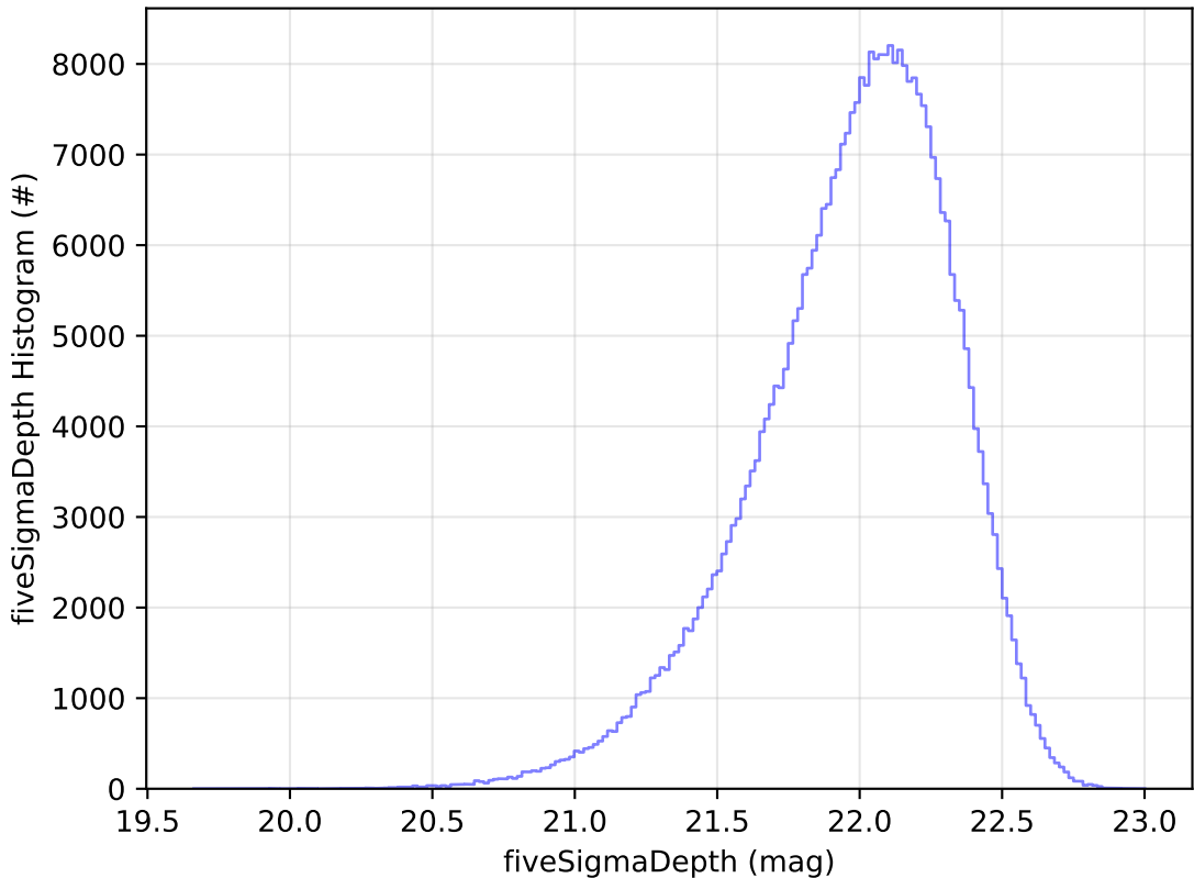
too_elab_2yr_r128_d3_griz_v3.4_10yrs y: fiveSigmaDepth Histogram
