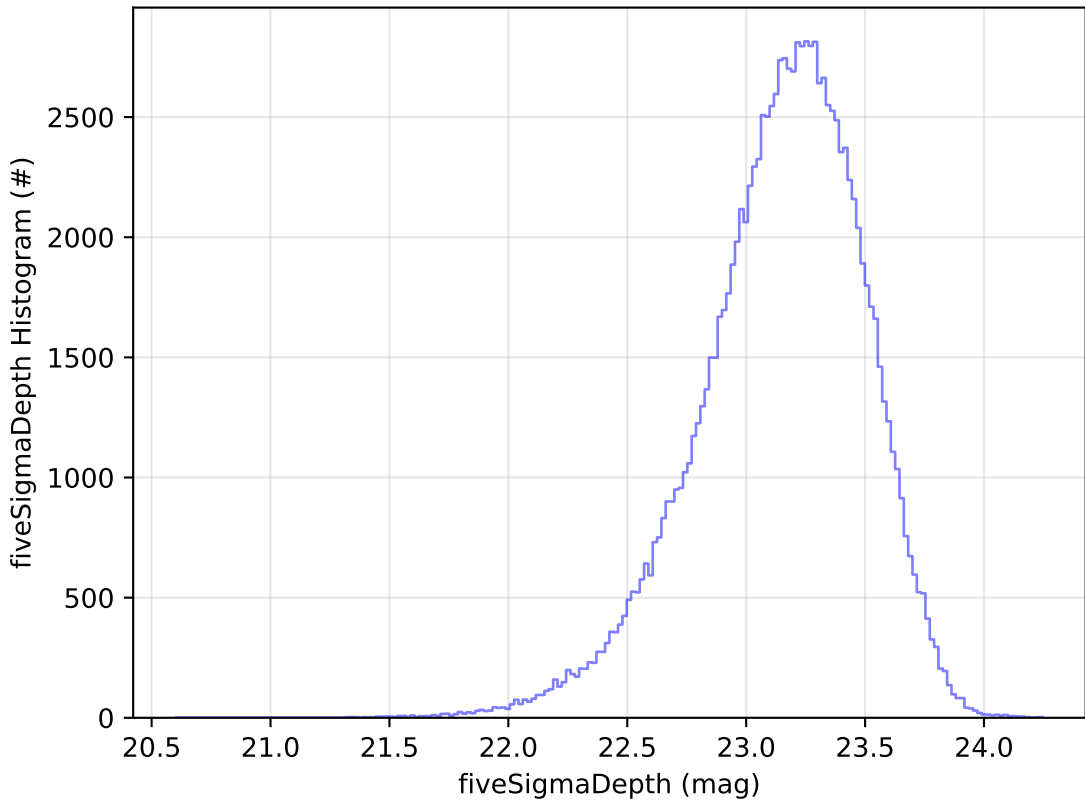
too_elab_2yr_r128_d3_griz_v3.4_10yrs u: fiveSigmaDepth Histogram
