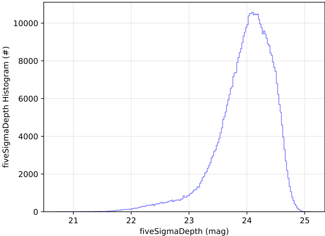
too_elab_2yr_r128_d3_griz_v3.4_10yrs r: fiveSigmaDepth Histogram
