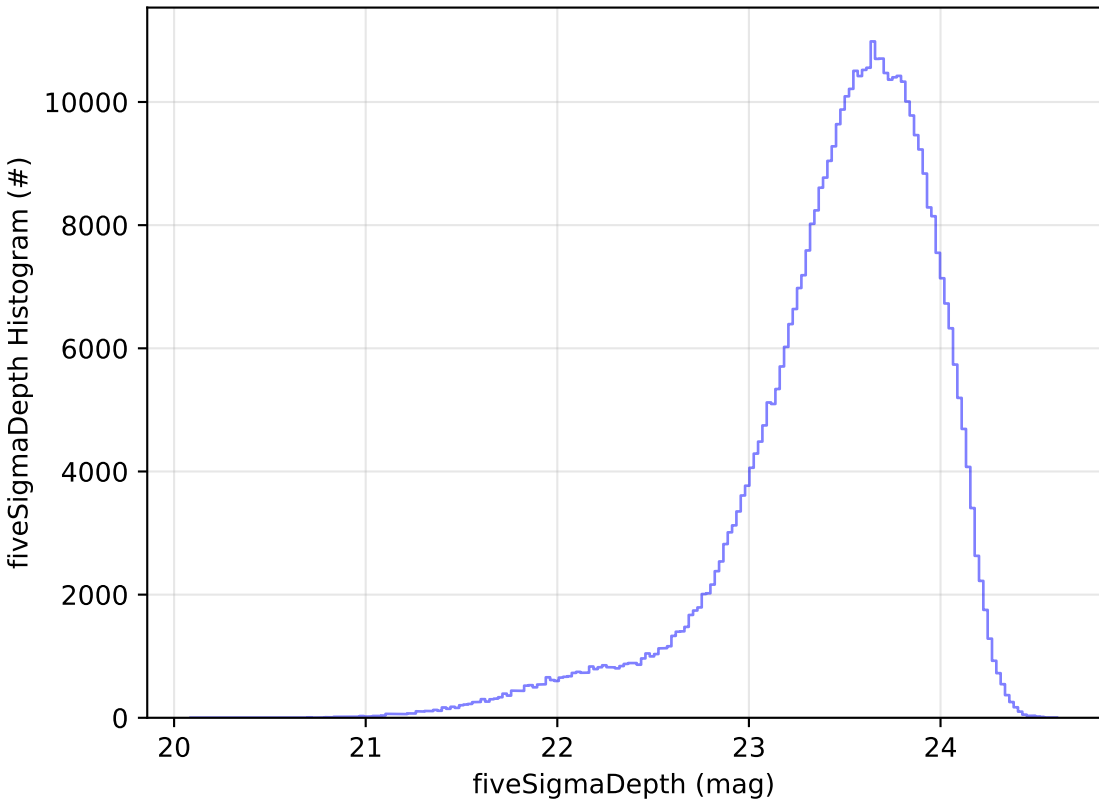
too_elab_2yr_r128_d3_griz_v3.4_10yrs i: fiveSigmaDepth Histogram
