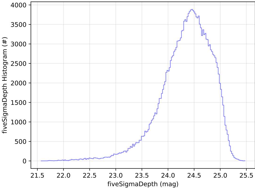
too_elab_2yr_r128_d3_griz_v3.4_10yrs g: fiveSigmaDepth Histogram
