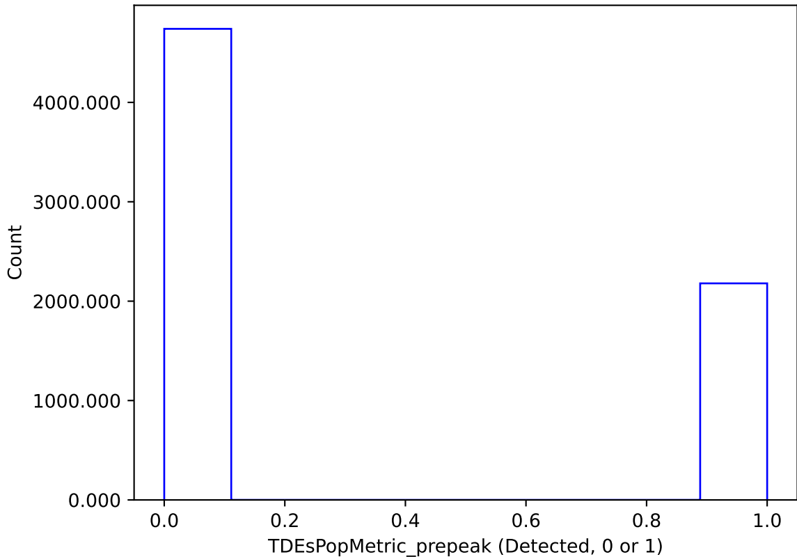
too_elab_2yr_r128_d3_griz_v3.4_10yrs : TDEsPopMetric_prepeak
