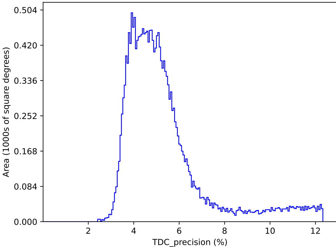
too_elab_2yr_r128_d3_griz_v3.4_10yrs : TDC_precision
