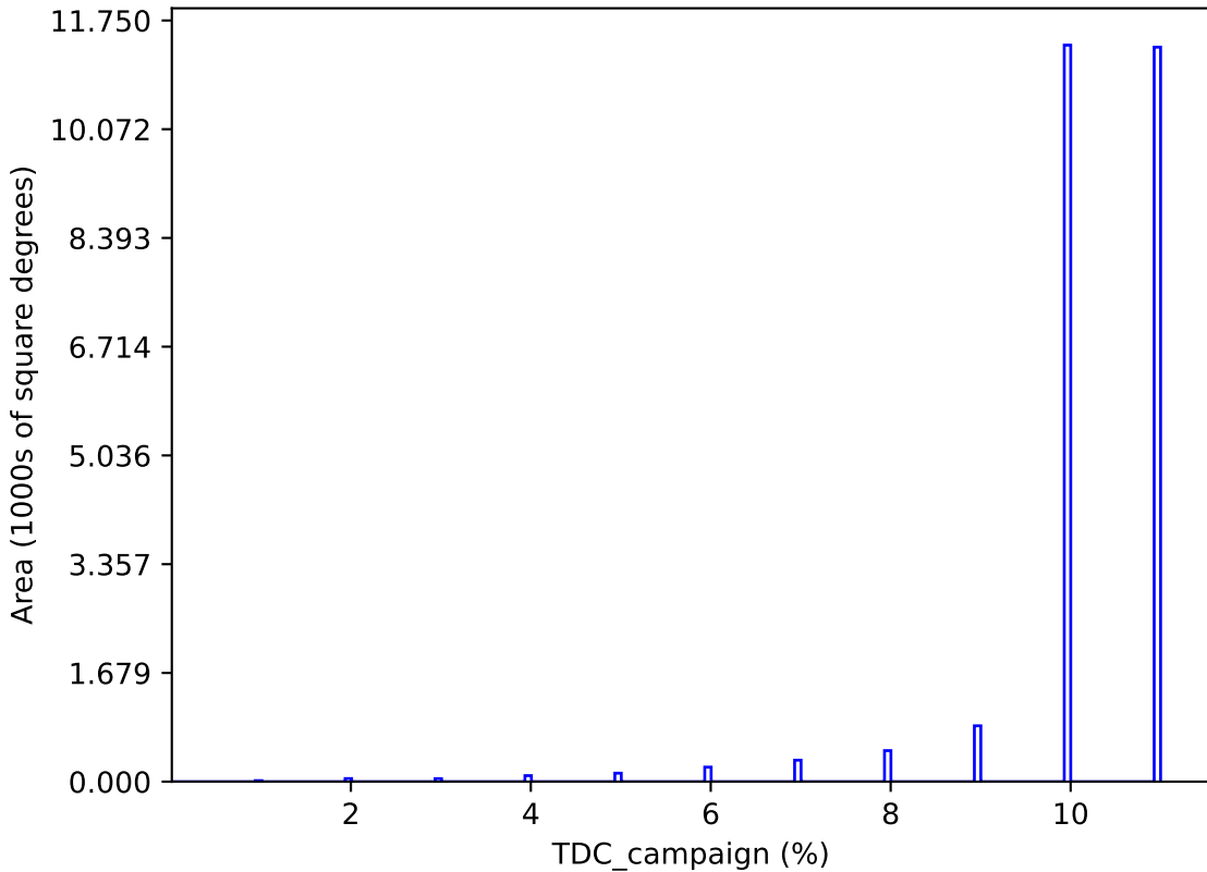
too_elab_2yr_r128_d3_griz_v3.4_10yrs : TDC_campaign
