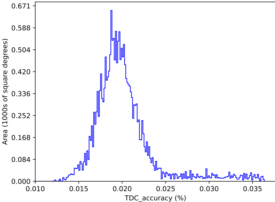
too_elab_2yr_r128_d3_griz_v3.4_10yrs : TDC_accuracy
