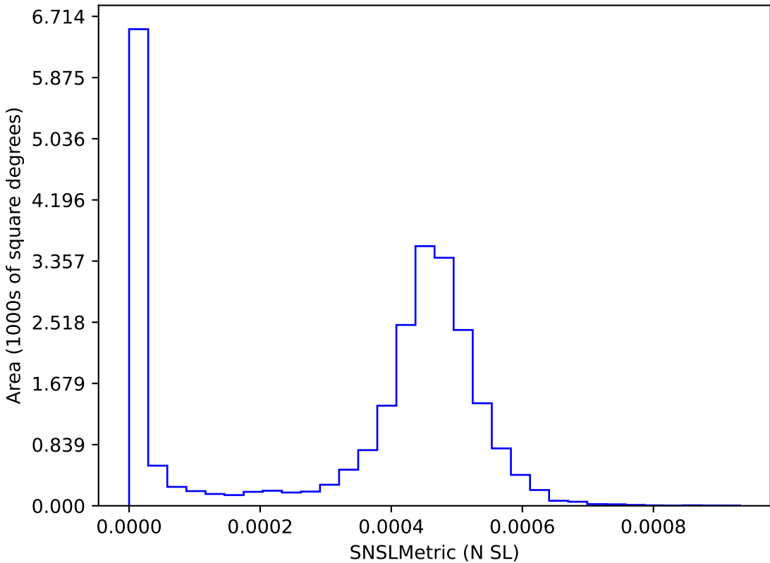
too_elab_2yr_r128_d3_griz_v3.4_10yrs : SNSLMetric
