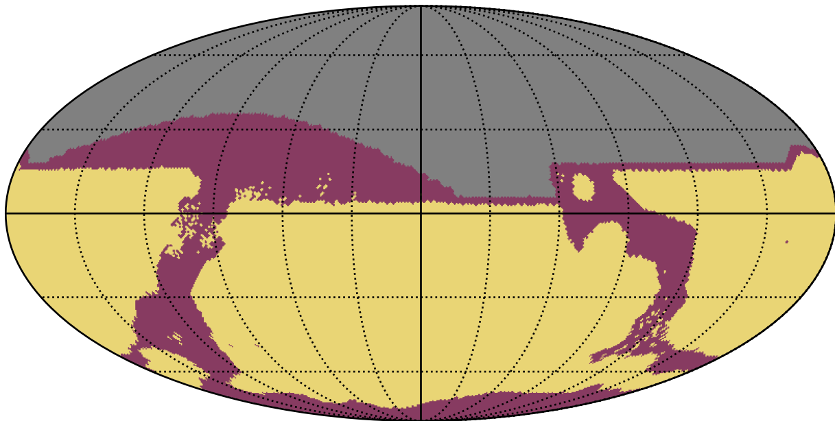
too_elab_2yr_r128_d3_griz_v3.4_10yrs : RapidRevisits
