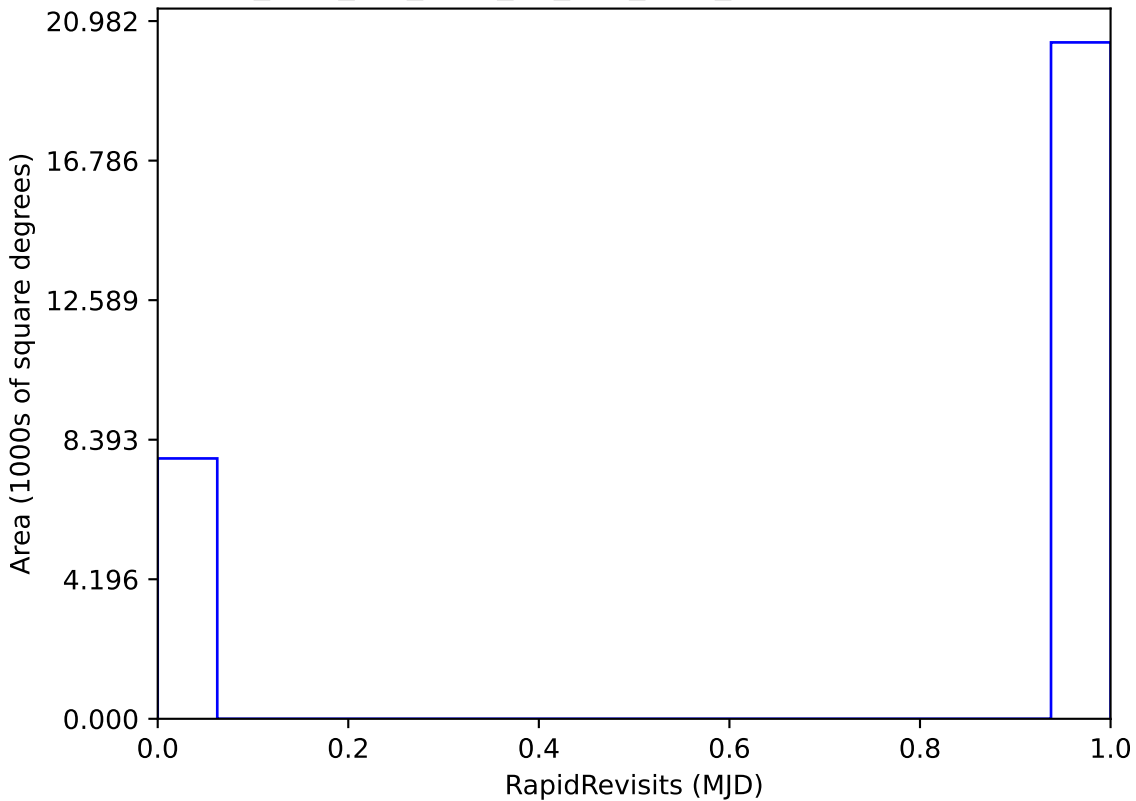
too_elab_2yr_r128_d3_griz_v3.4_10yrs : RapidRevisits
