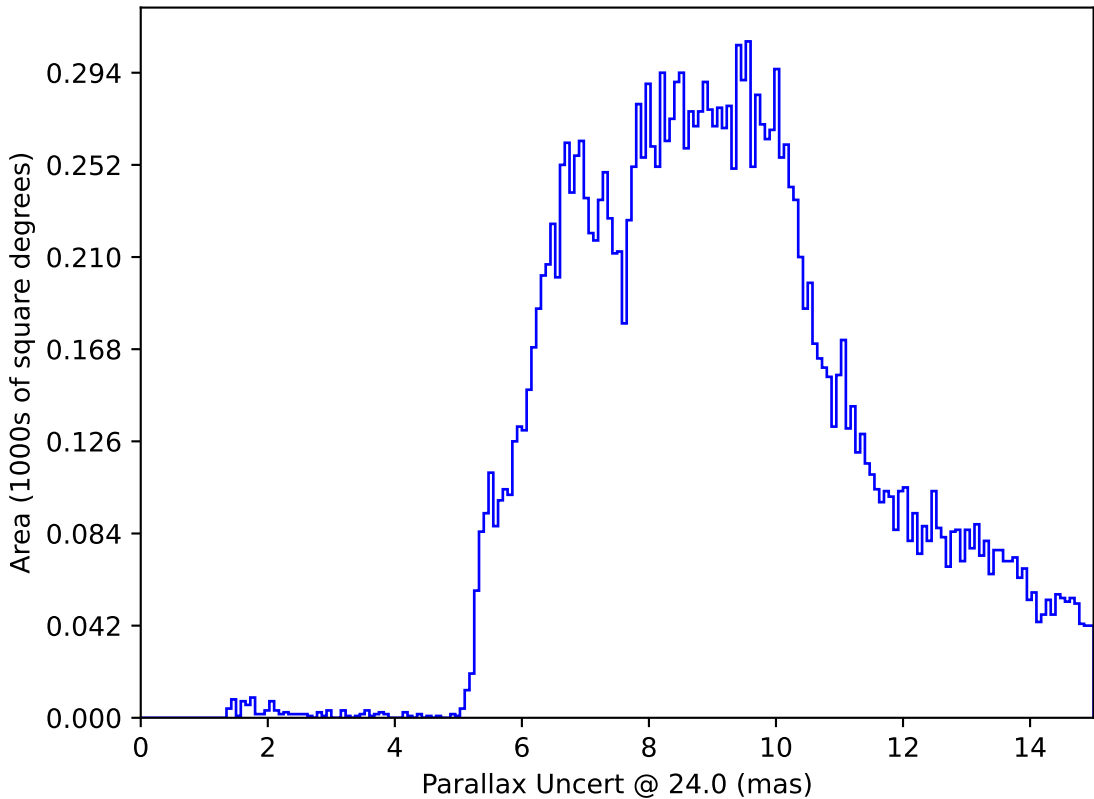
too_elab_2yr_r128_d3_griz_v3.4_10yrs : Parallax Uncert @ 24.0
