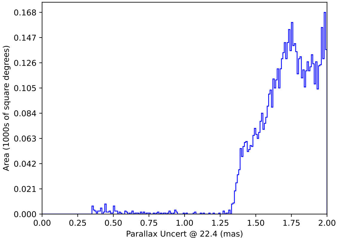
too_elab_2yr_r128_d3_griz_v3.4_10yrs : Parallax Uncert @ 22.4
