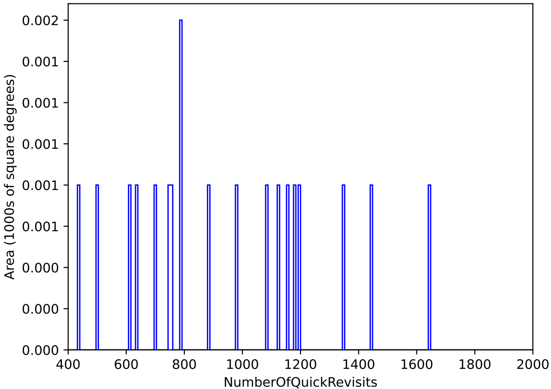
too_elab_2yr_r128_d3_griz_v3.4_10yrs : NumberOfQuickRevisits
