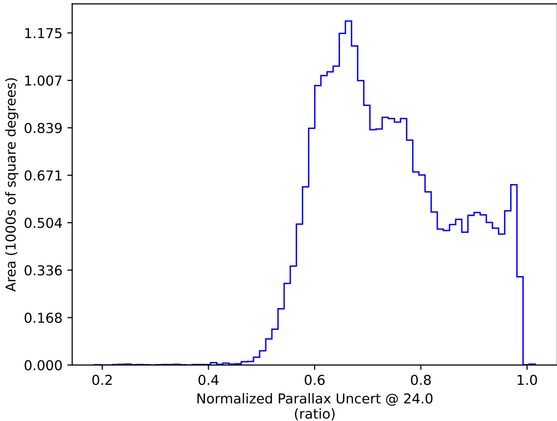
too_elab_2yr_r128_d3_griz_v3.4_10yrs : Normalized Parallax Uncert @ 24.0
