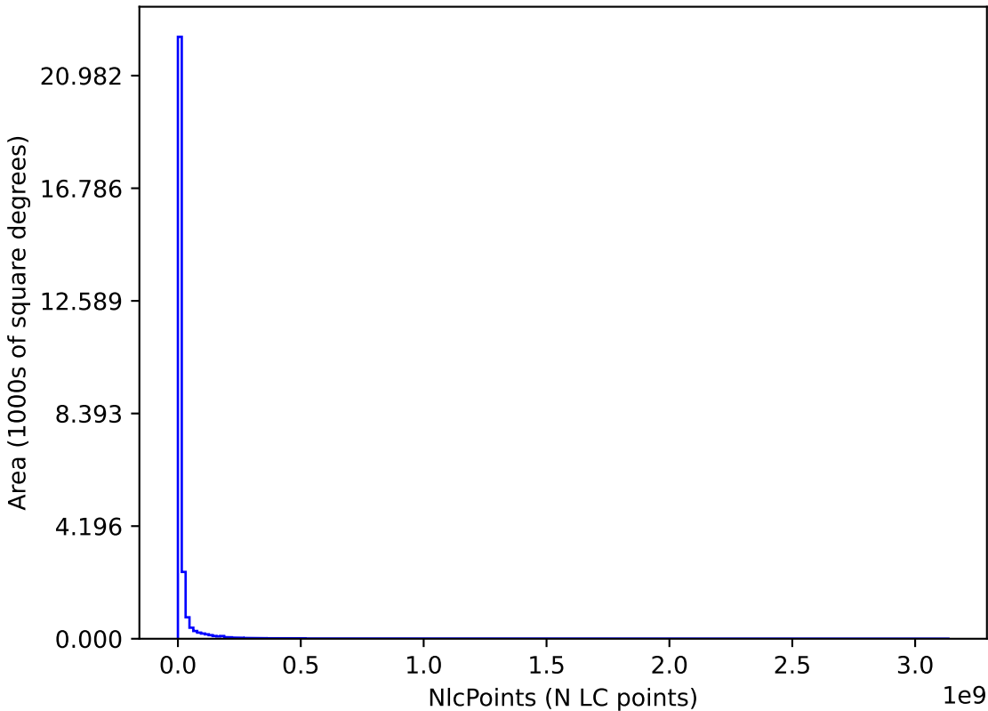
too_elab_2yr_r128_d3_griz_v3.4_10yrs : NlcPoints
