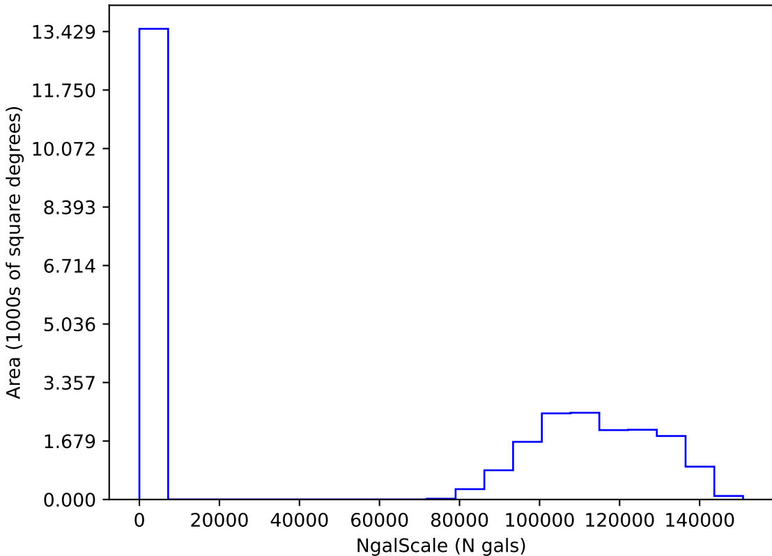
too_elab_2yr_r128_d3_griz_v3.4_10yrs i: NgalScale
