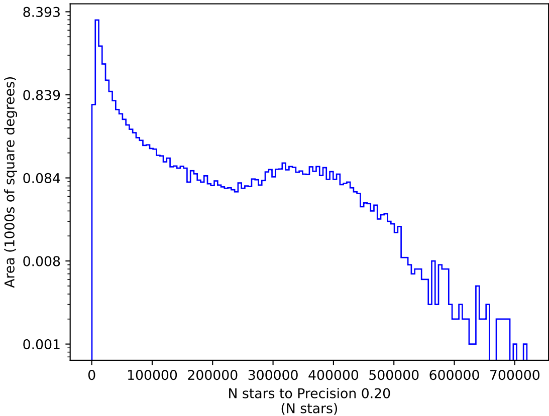
too_elab_2yr_r128_d3_griz_v3.4_10yrs y: N stars to Precision 0.20
