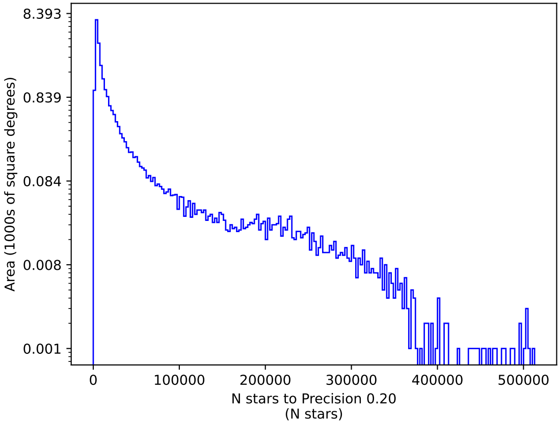
too_elab_2yr_r128_d3_griz_v3.4_10yrs u: N stars to Precision 0.20
