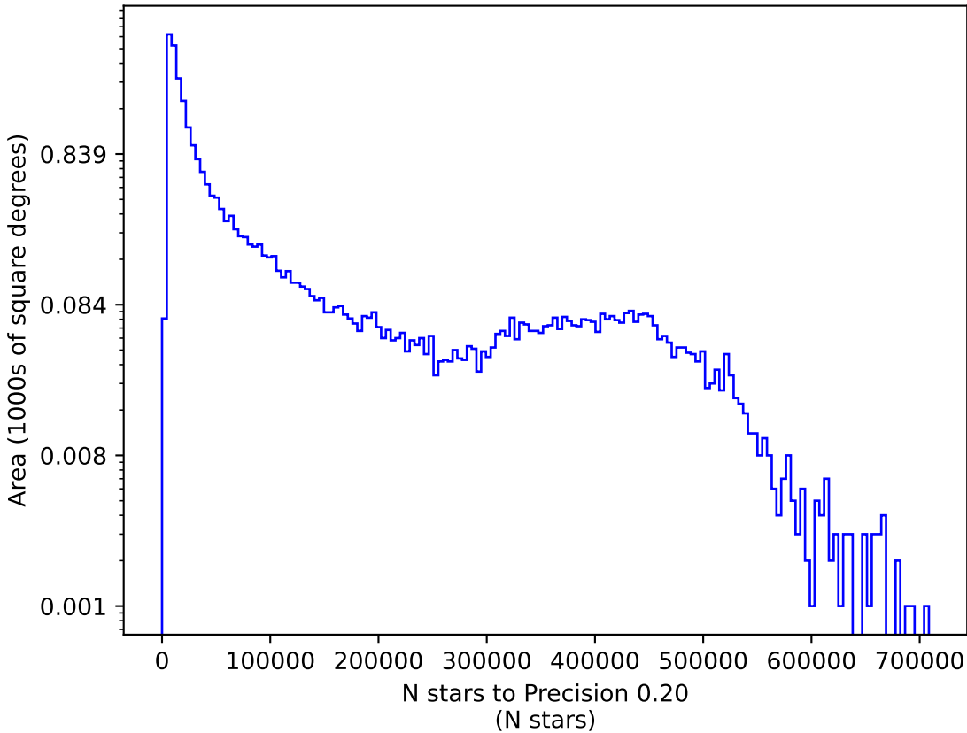
too_elab_2yr_r128_d3_griz_v3.4_10yrs r: N stars to Precision 0.20
