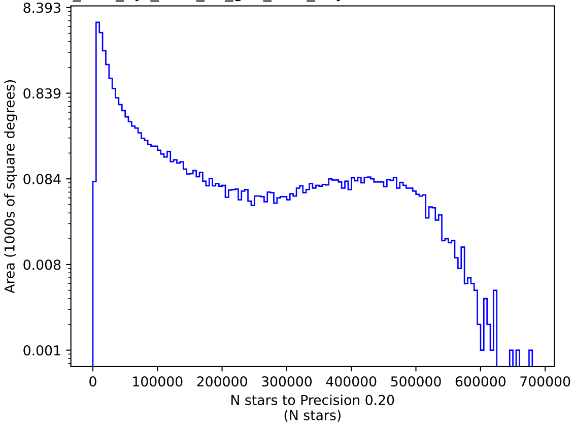
too_elab_2yr_r128_d3_griz_v3.4_10yrs i: N stars to Precision 0.20
