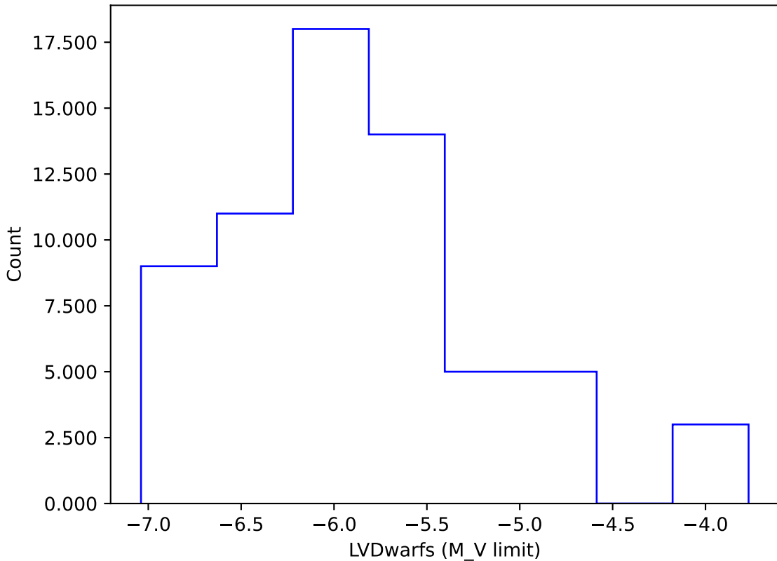
too_elab_2yr_r128_d3_griz_v3.4_10yrs gi: LVDwarfs
