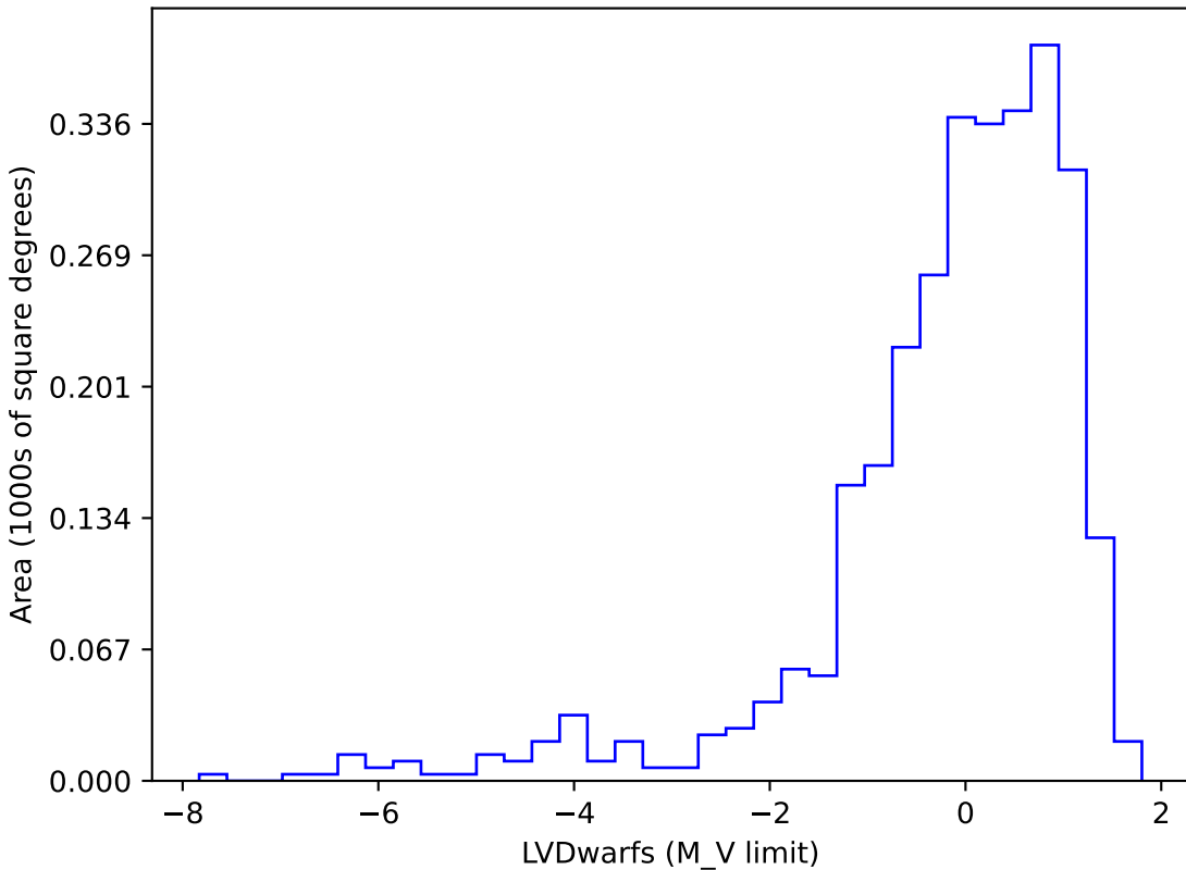
too_elab_2yr_r128_d3_griz_v3.4_10yrs gi SCP: LVDwarfs
