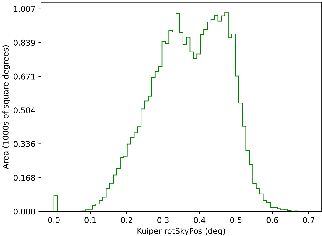
too_elab_2yr_r128_d3_griz_v3.4_10yrs g: Kuiper rotSkyPos
