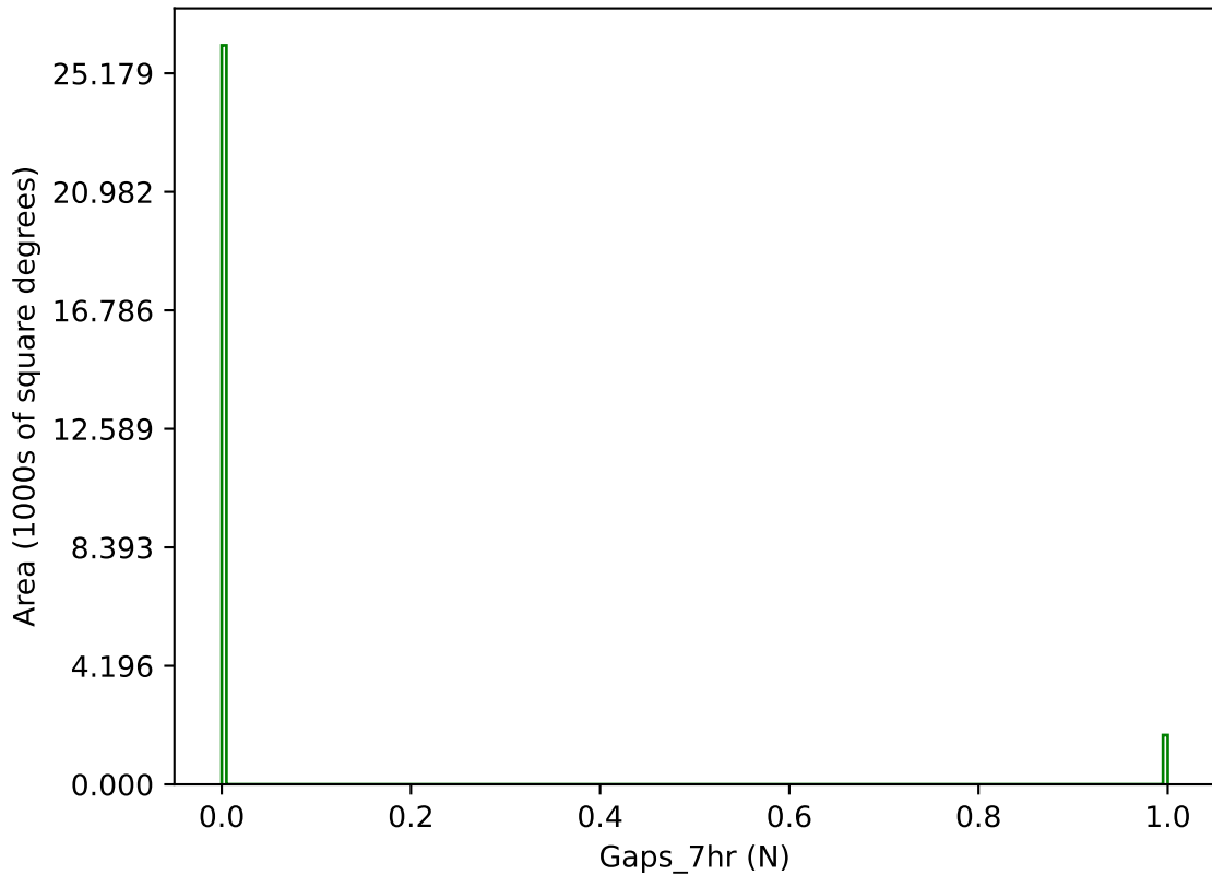
too_elab_2yr_r128_d3_griz_v3.4_10yrs g band: Gaps_7hr
