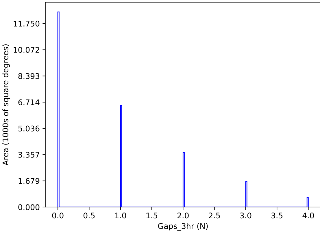
too_elab_2yr_r128_d3_griz_v3.4_10yrs y band: Gaps_3hr
