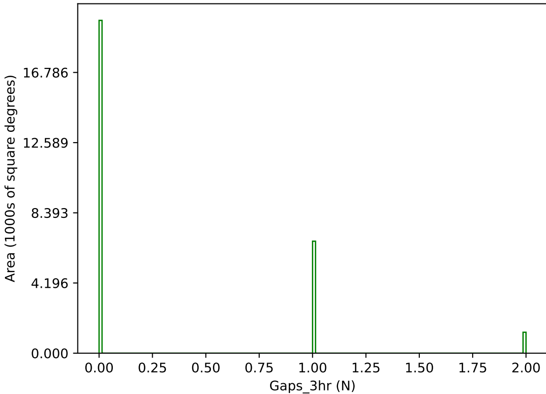
too_elab_2yr_r128_d3_griz_v3.4_10yrs g band: Gaps_3hr
