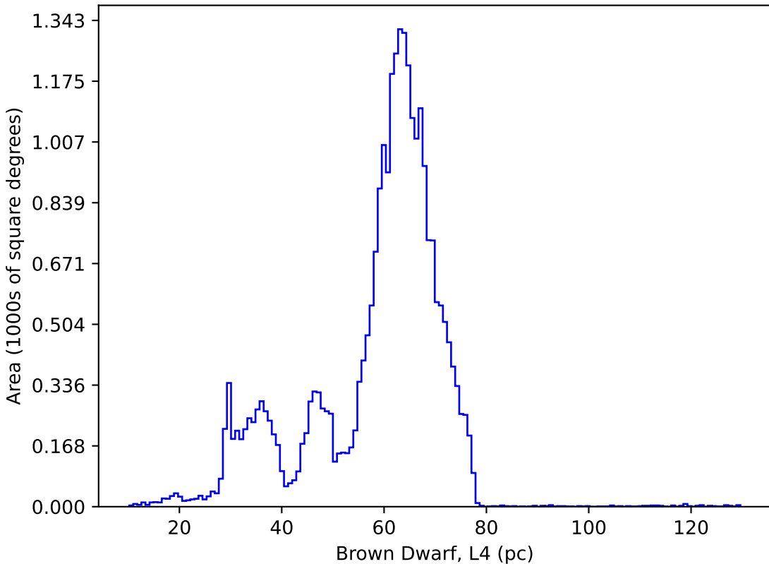
too_elab_2yr_r128_d3_griz_v3.4_10yrs : Brown Dwarf, L4
