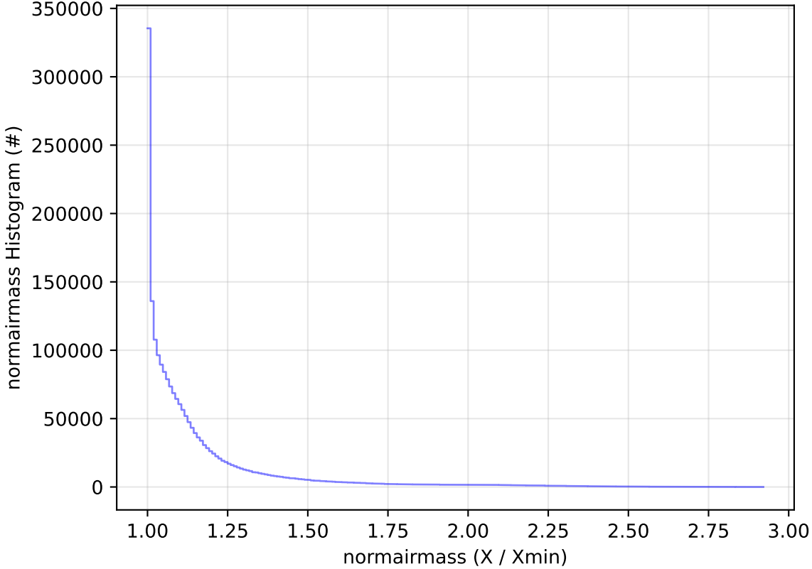
too_elab_2yr_r128_d3_griz_v3.4_10yrs WFD all bands: normairmass Histogram
