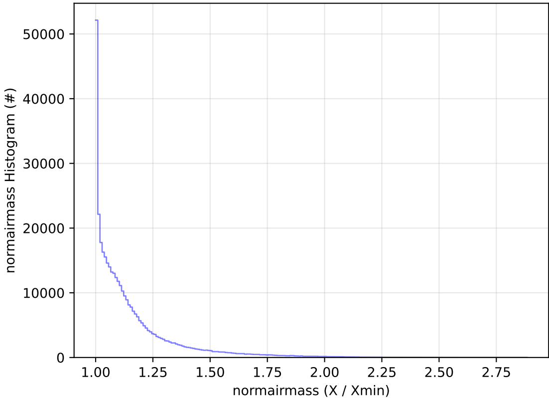
too_elab_2yr_r128_d3_griz_v3.4_10yrs All sky y band: normairmass Histogram
