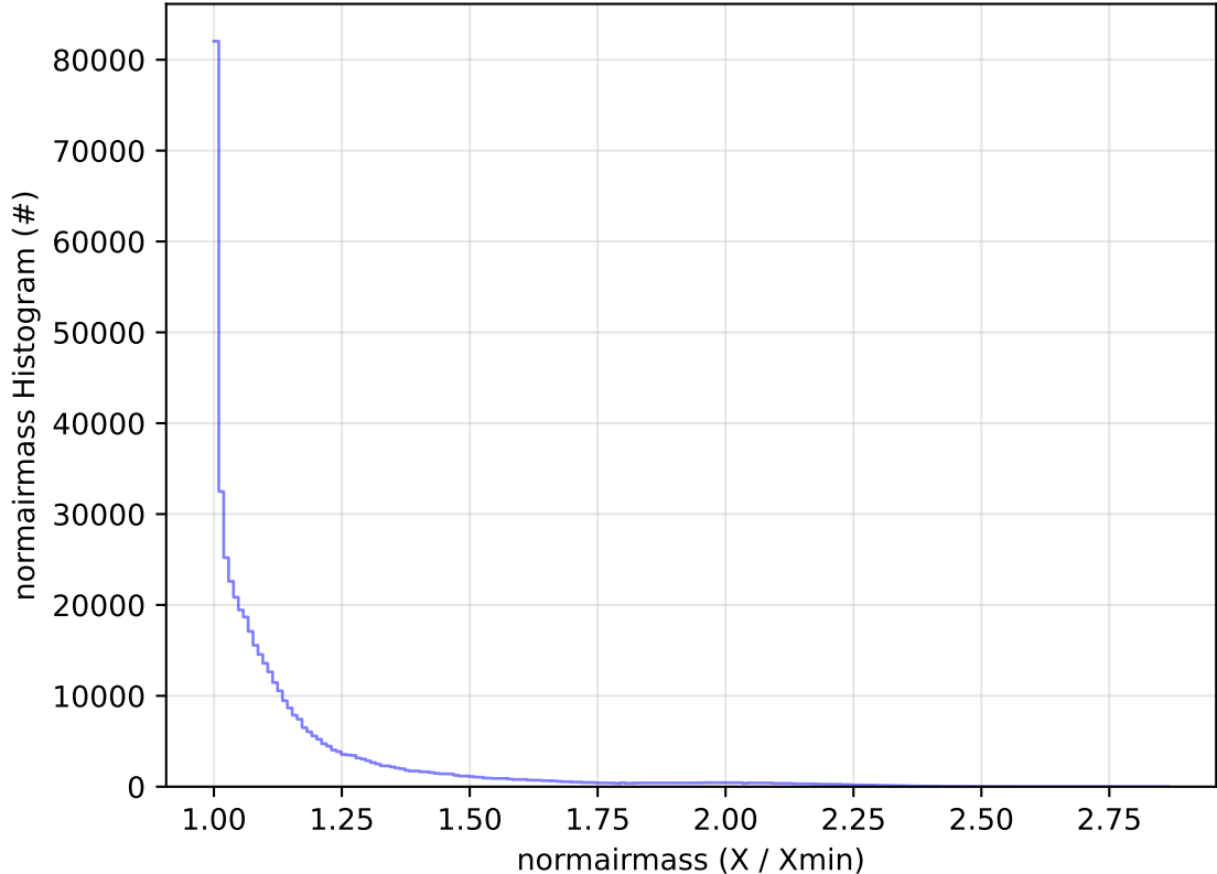
too_elab_2yr_r128_d3_griz_v3.4_10yrs All sky r band: normairmass Histogram
