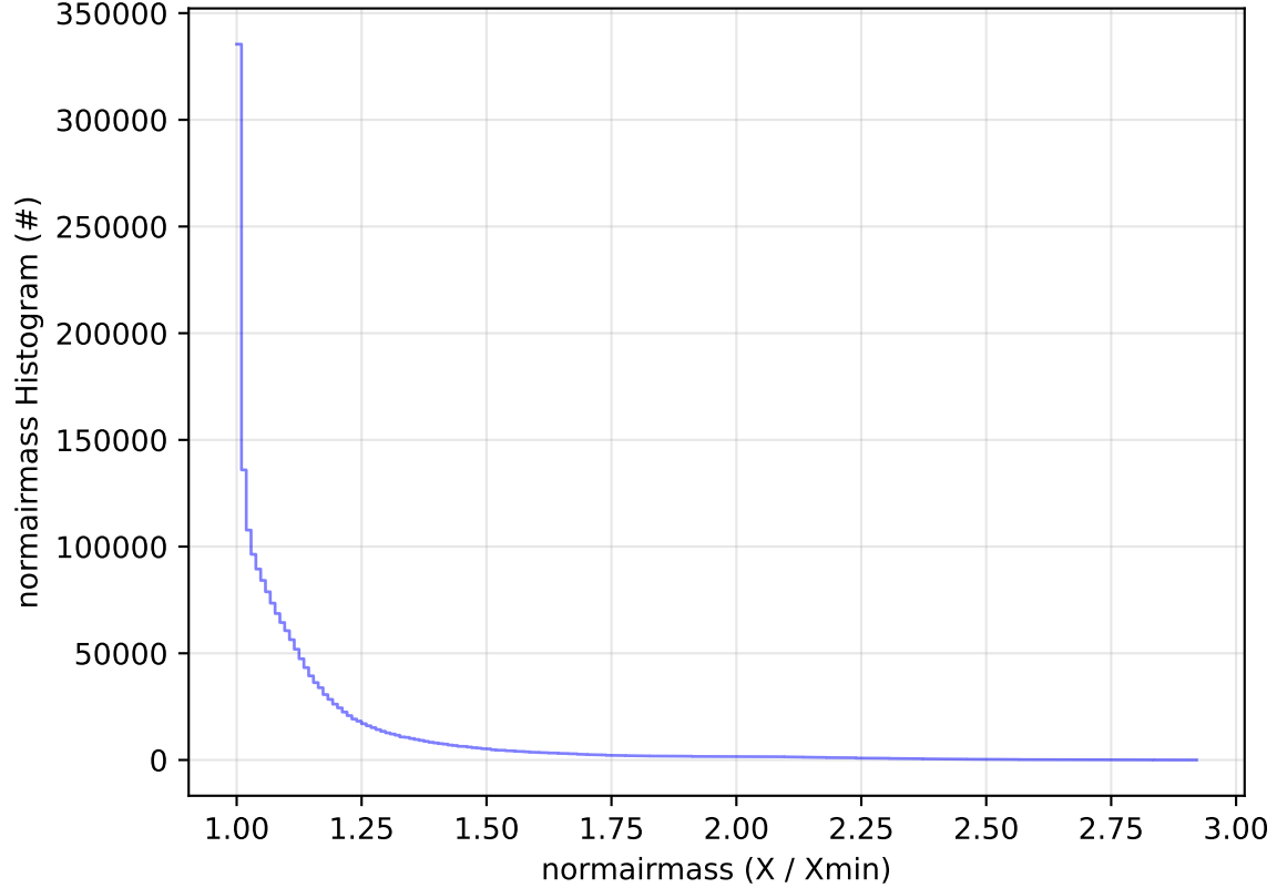
too_elab_2yr_r128_d3_griz_v3.4_10yrs All sky all bands: normairmass Histogram
