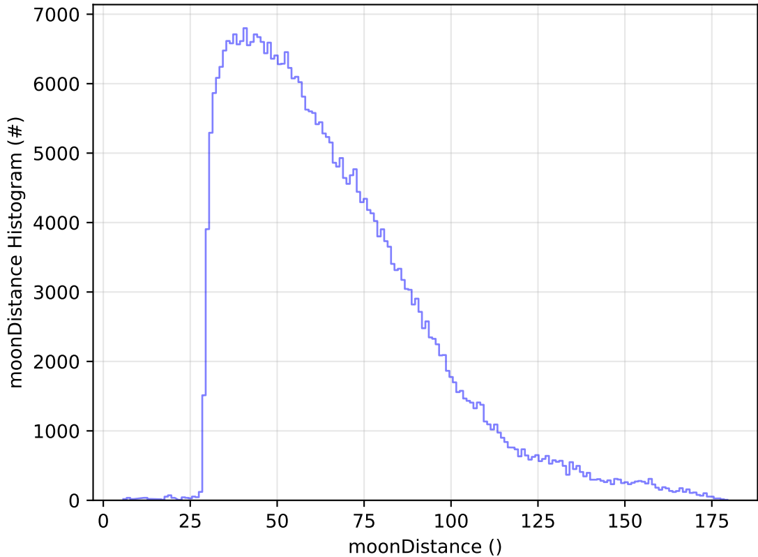
too_elab_2yr_r128_d3_griz_v3.4_10yrs WFD y band: moonDistance Histogram
