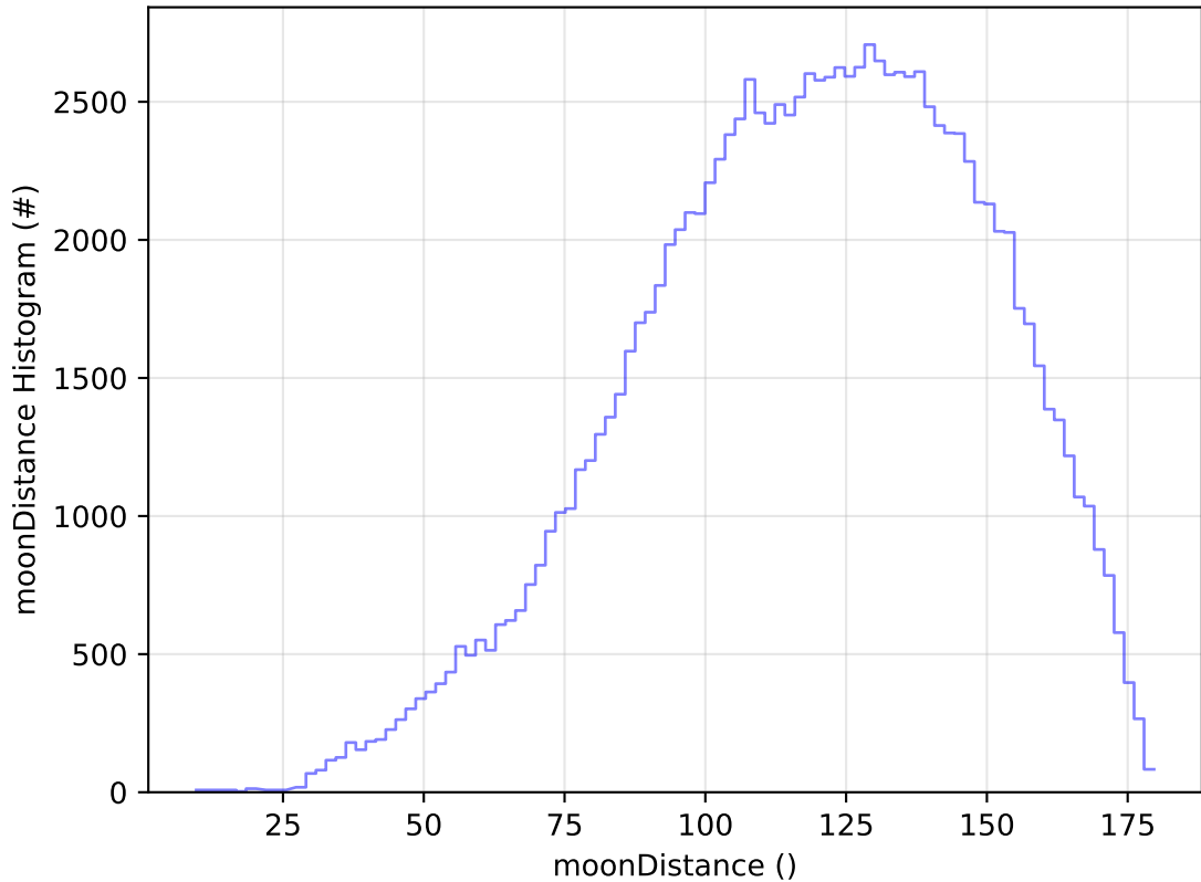
too_elab_2yr_r128_d3_griz_v3.4_10yrs WFD u band: moonDistance Histogram
