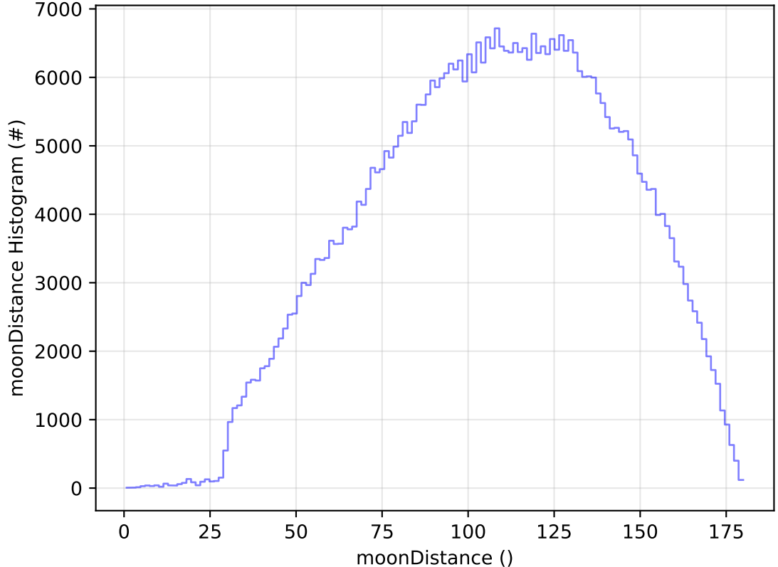
too_elab_2yr_r128_d3_griz_v3.4_10yrs WFD r band: moonDistance Histogram
