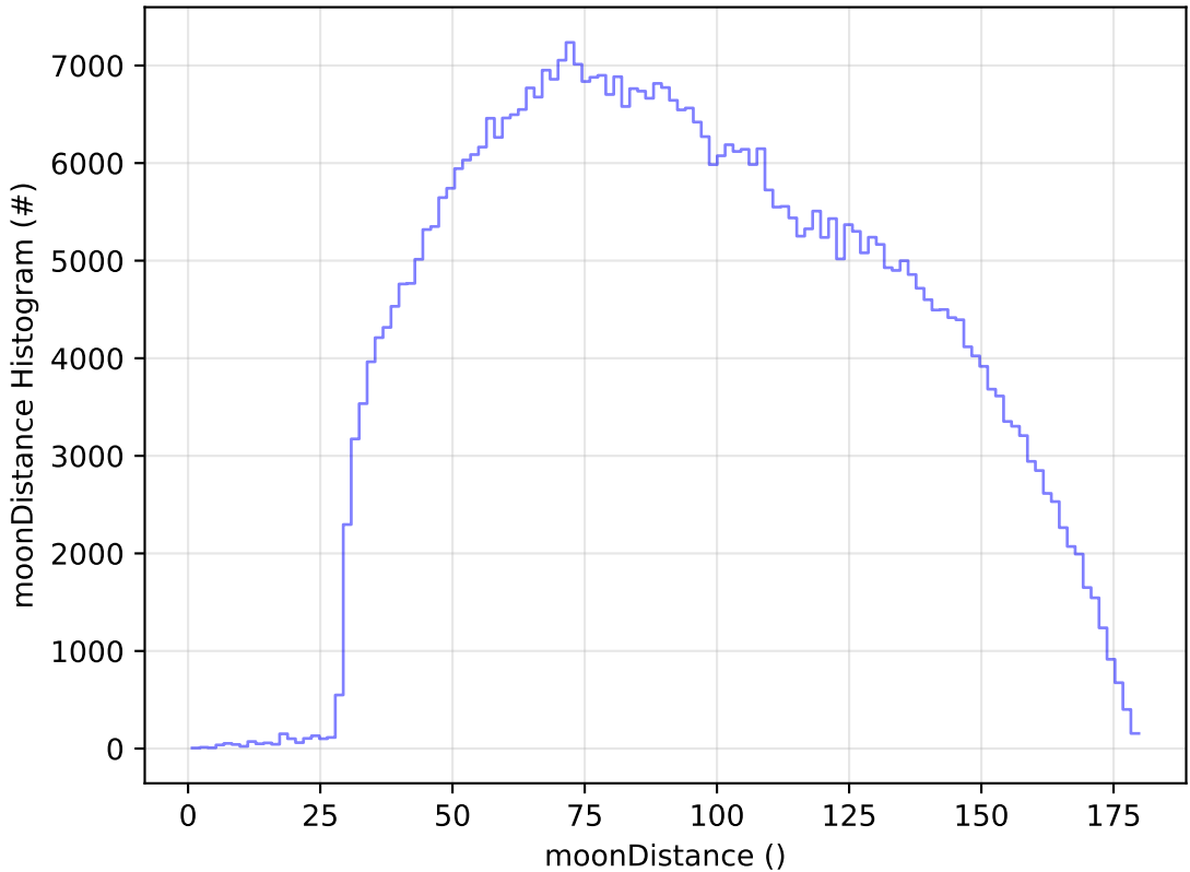
too_elab_2yr_r128_d3_griz_v3.4_10yrs WFD i band: moonDistance Histogram
