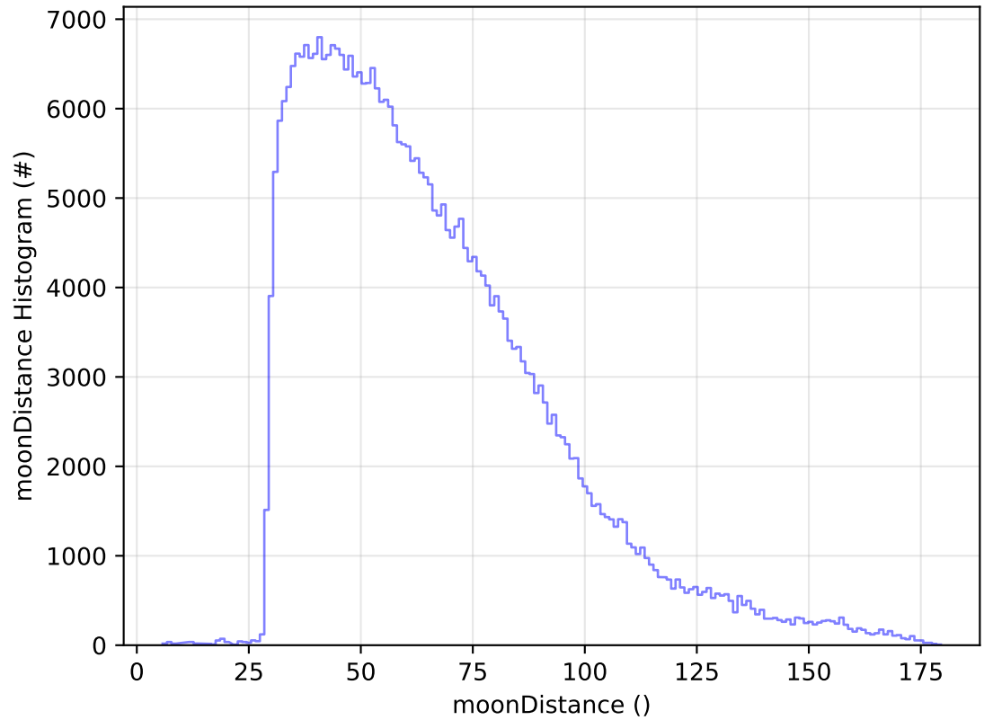
too_elab_2yr_r128_d3_griz_v3.4_10yrs All sky y band: moonDistance Histogram
