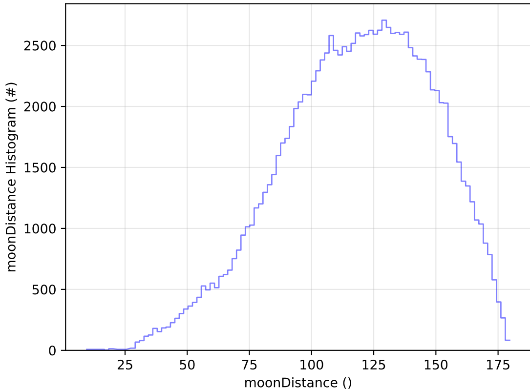
too_elab_2yr_r128_d3_griz_v3.4_10yrs All sky u band: moonDistance Histogram
