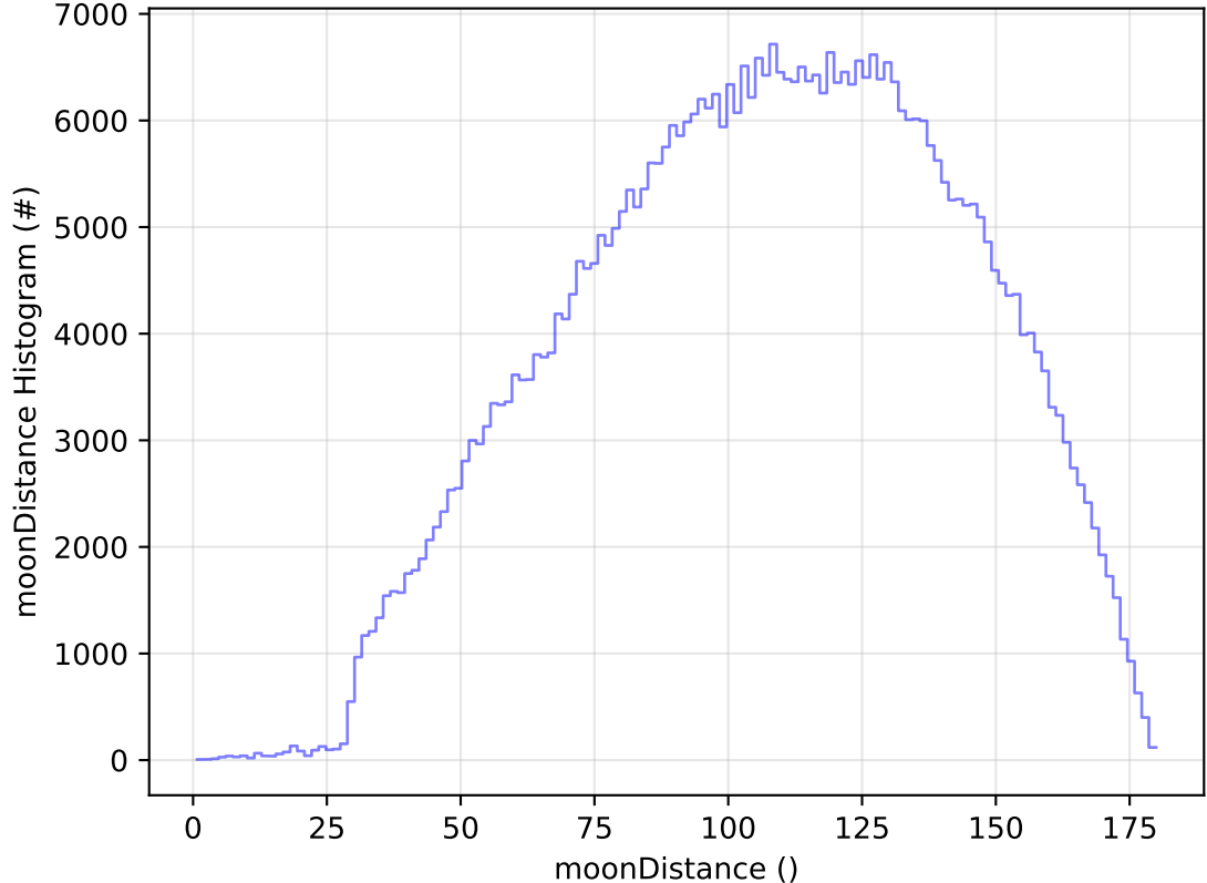
too_elab_2yr_r128_d3_griz_v3.4_10yrs All sky r band: moonDistance Histogram
