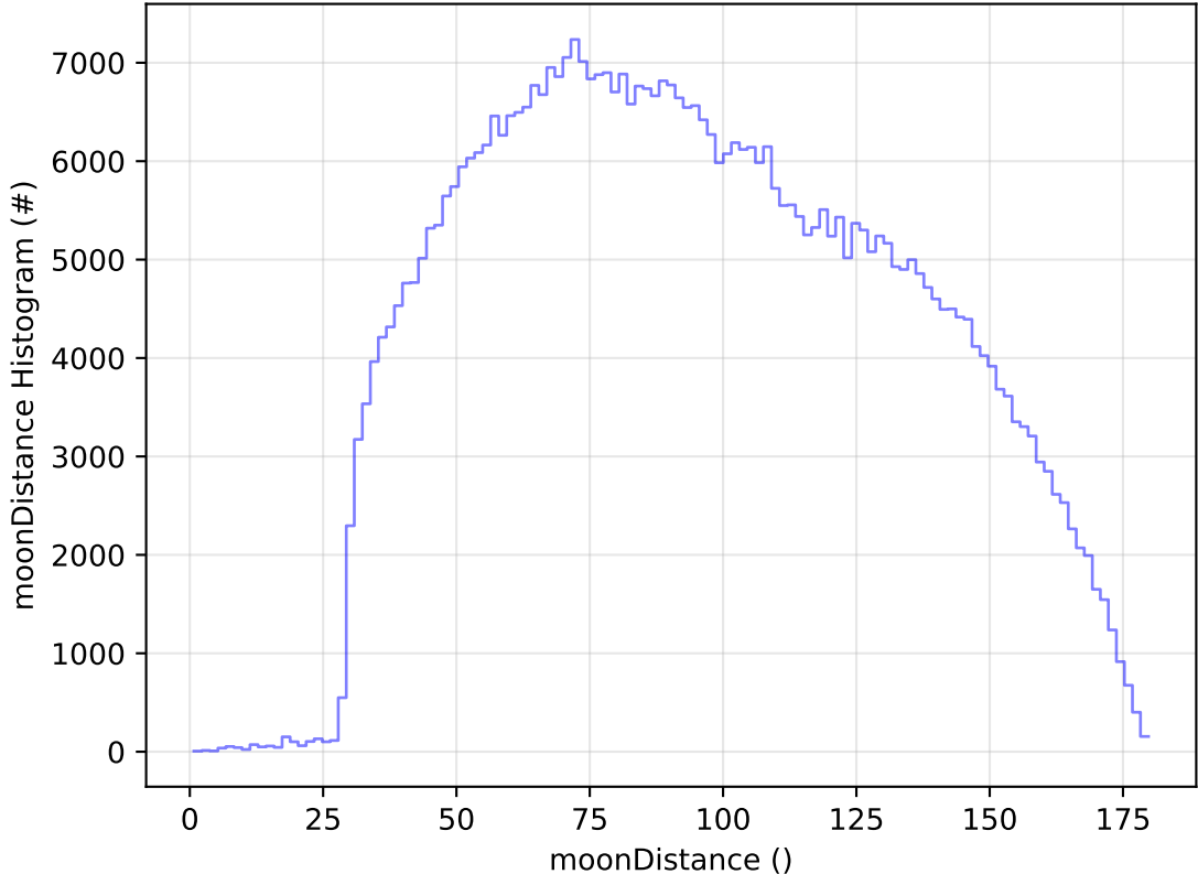
too_elab_2yr_r128_d3_griz_v3.4_10yrs All sky i band: moonDistance Histogram
