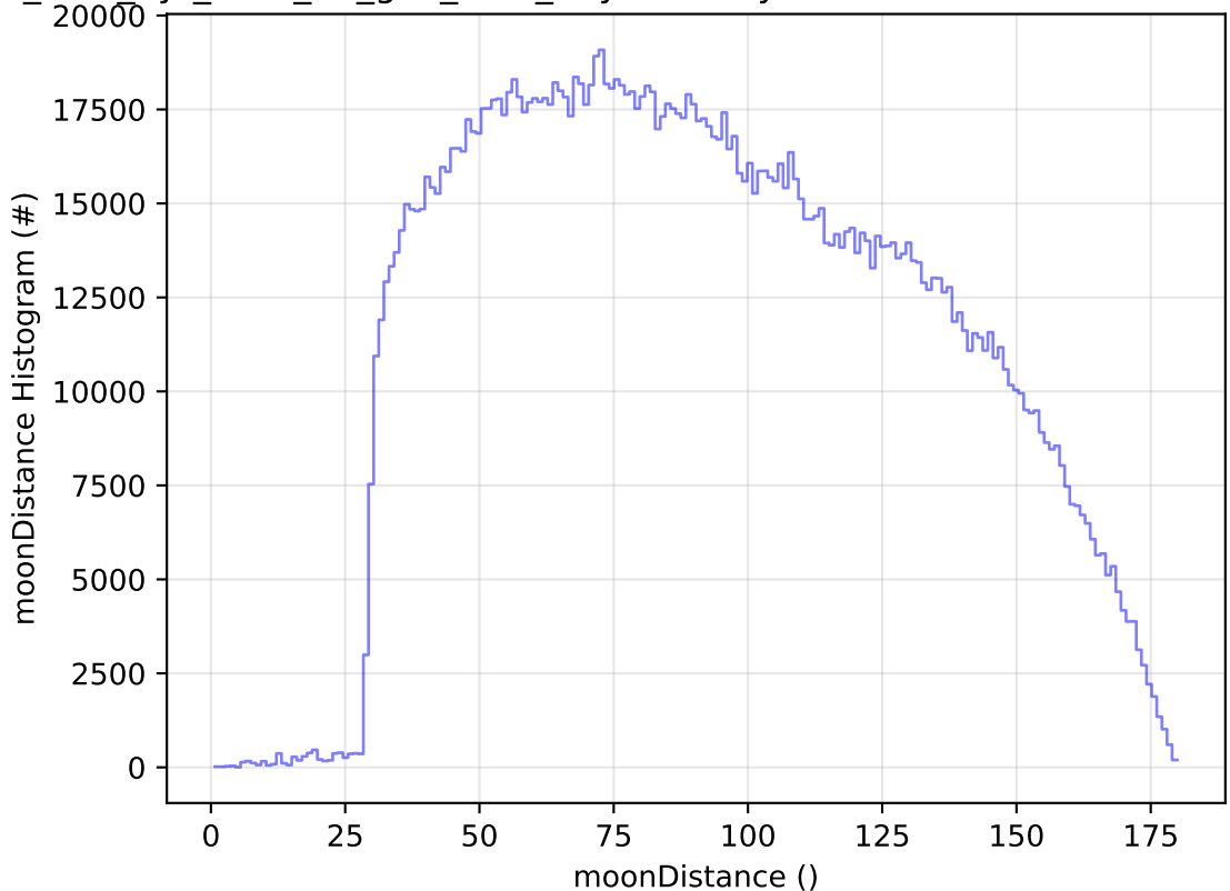
too_elab_2yr_r128_d3_griz_v3.4_10yrs All sky all bands: moonDistance Histogram
