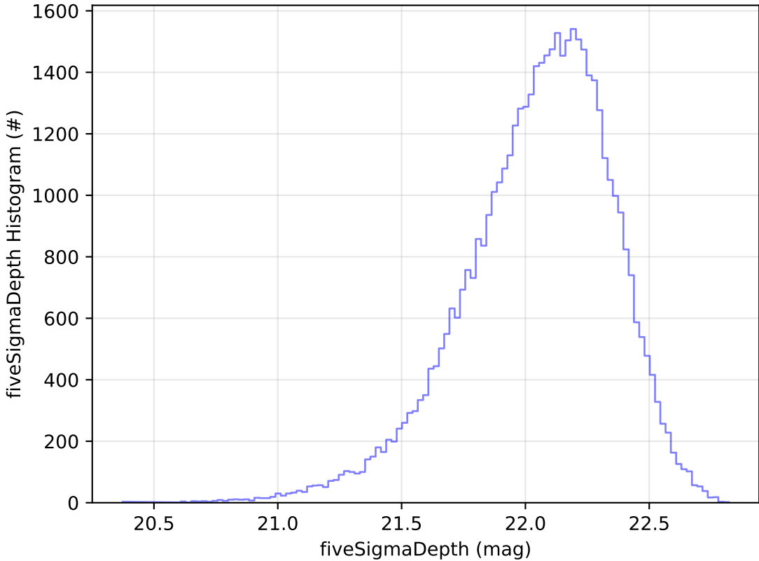
too_elab_2yr_r128_d3_griz_v3.4_10yrs Yr 1 y band: fiveSigmaDepth Histogram
