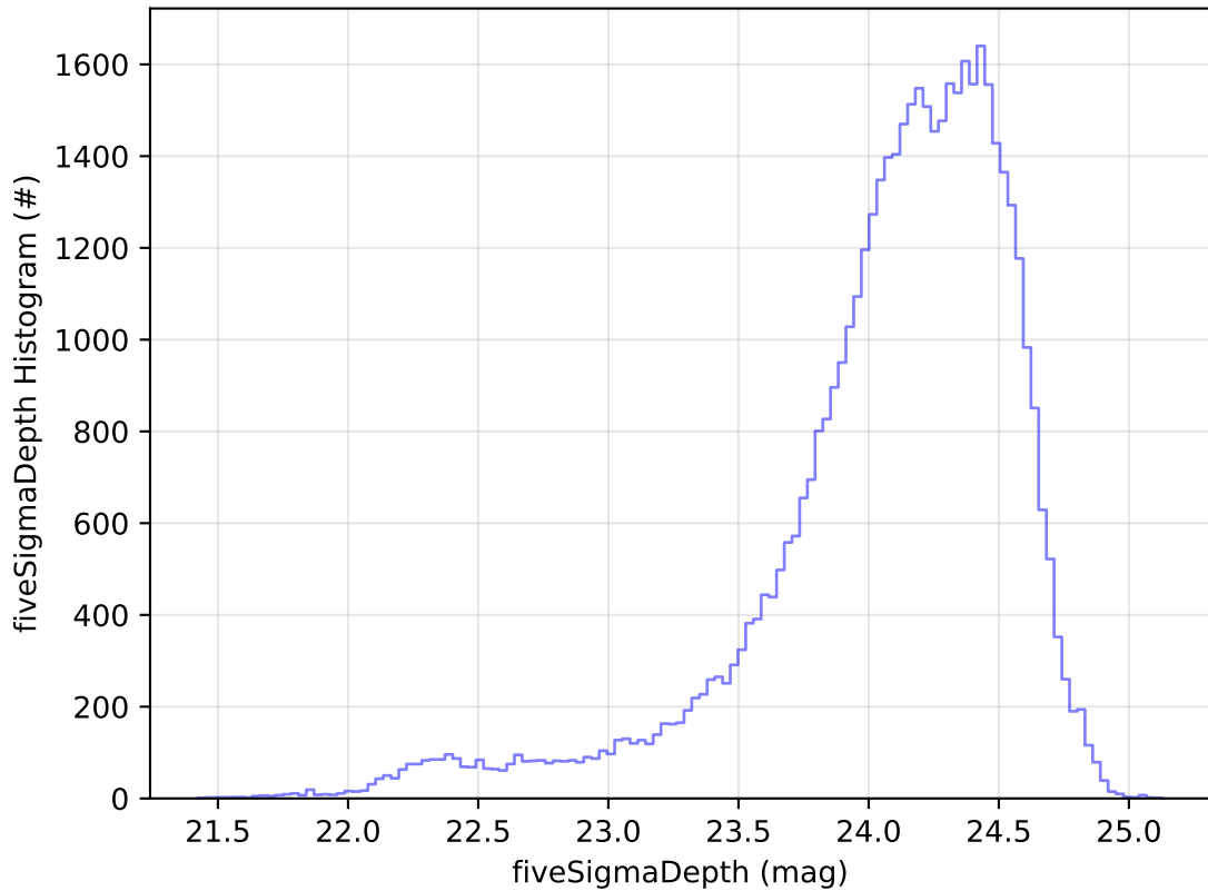
too_elab_2yr_r128_d3_griz_v3.4_10yrs Yr 1 r band: fiveSigmaDepth Histogram
