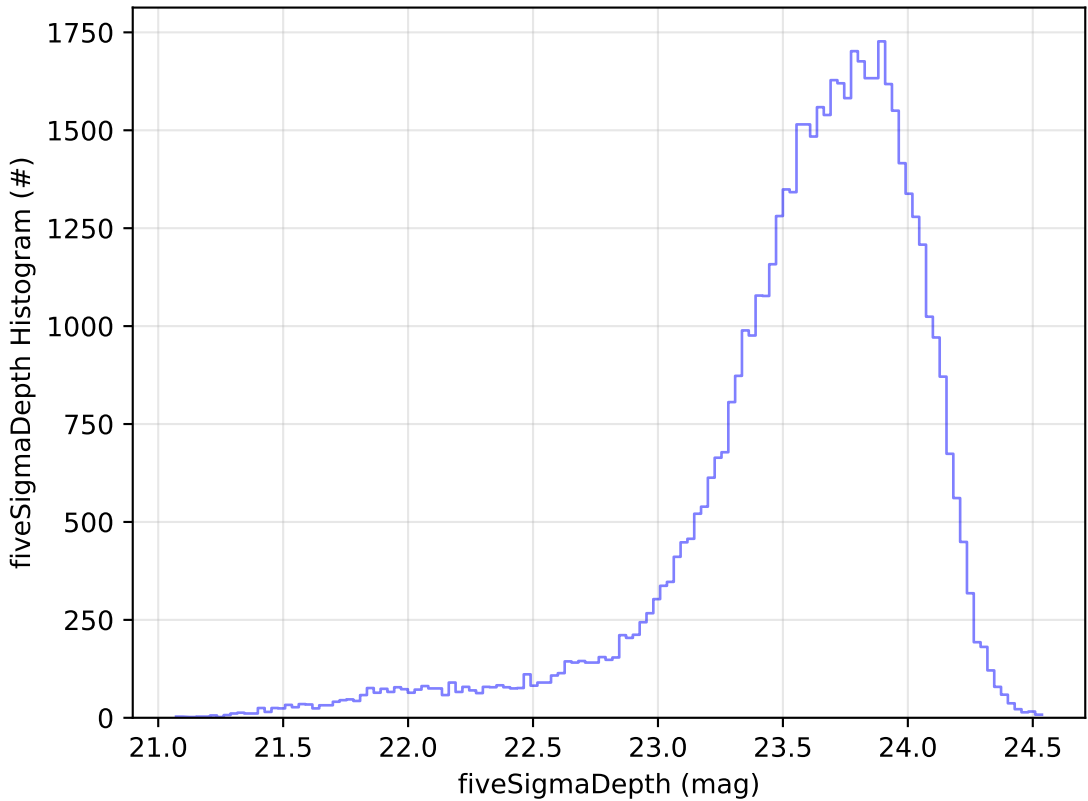
too_elab_2yr_r128_d3_griz_v3.4_10yrs Yr 1 i band: fiveSigmaDepth Histogram
