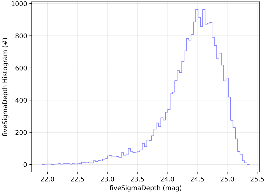
too_elab_2yr_r128_d3_griz_v3.4_10yrs Yr 1 g band: fiveSigmaDepth Histogram
