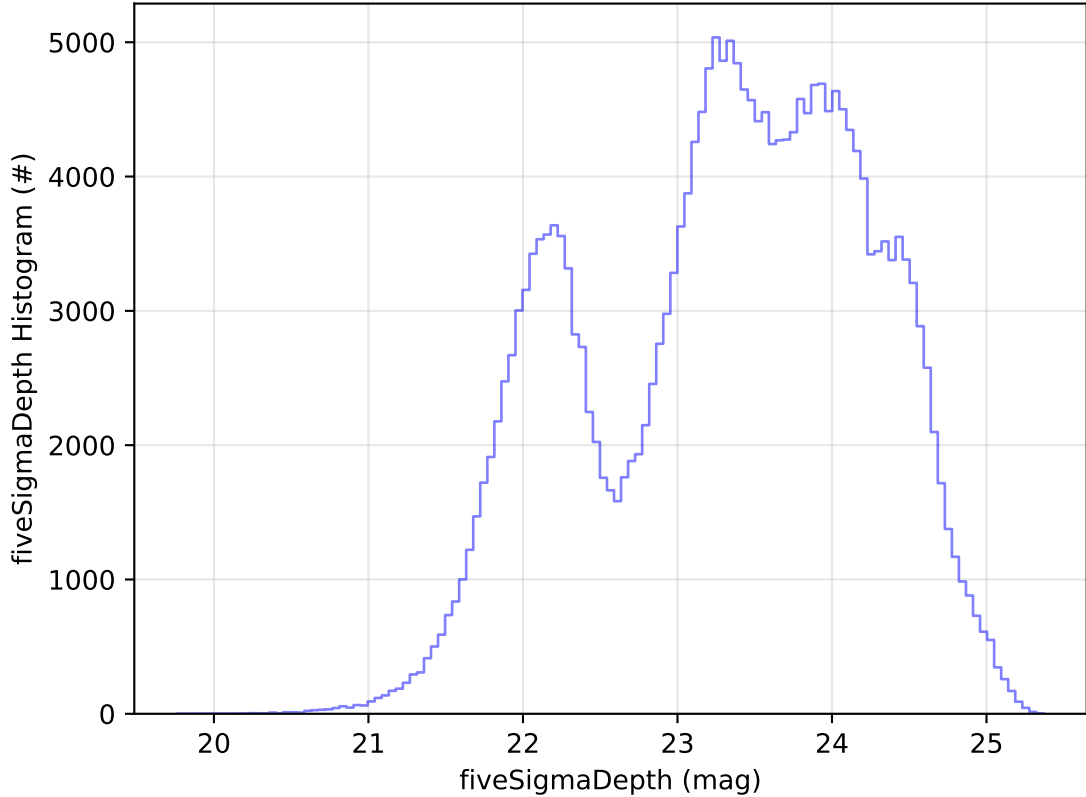
too_elab_2yr_r128_d3_griz_v3.4_10yrs Yr 1 all bands: fiveSigmaDepth Histogram
